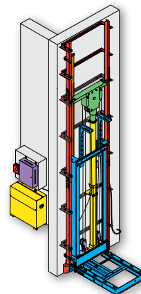
Excelelevator Roped Hydraulic Series 114 Capacity 1,000 lbs
